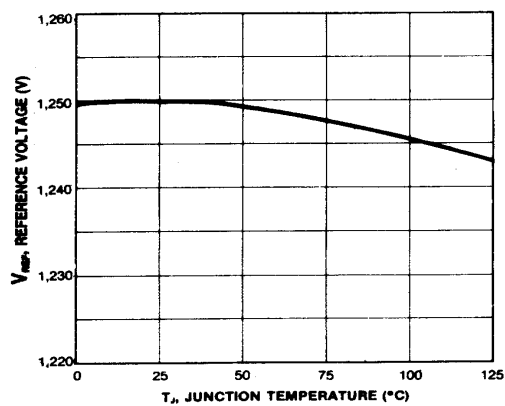
Figure 6. Temperature Stability
