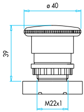
Acil Stop Ø 40 mm Emergency Stop Ø 40 mm
