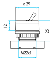
Mandallı Handle Button
