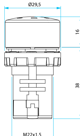
Monoblok Buzzer Monoblock Buzzer
