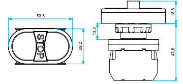
Üçüz Buton Triple, With Extended Stop
