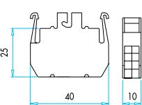
B Serisi Ampul Takılabilen Işıklı Blok Neon Lamp Mountable B Series Light Block
