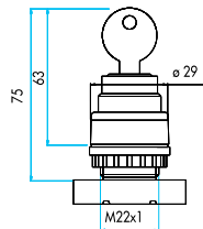
Anahtarlı Key Operated
