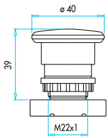
Mantar Mushroom, Spring Return
