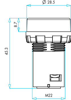
Sinyal (Düz Cam) Signal (Flat Glass)
