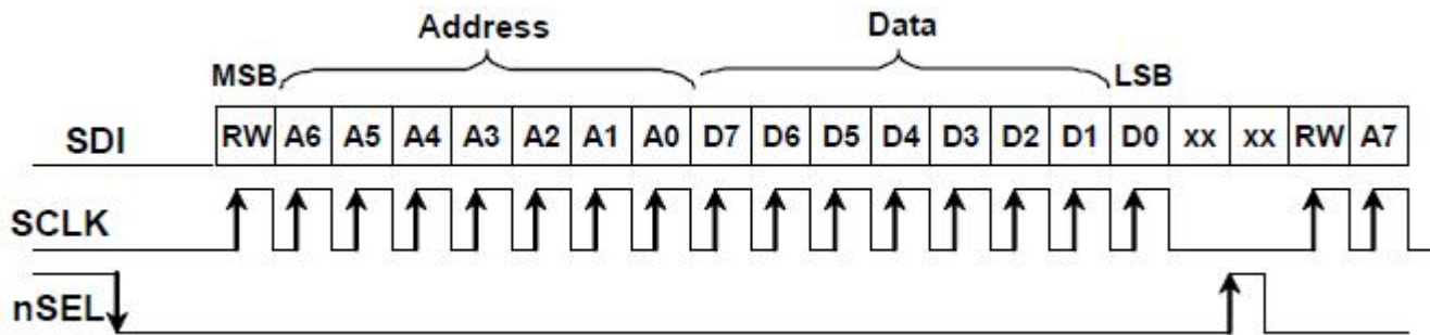
Figure 2. SPI Timing
