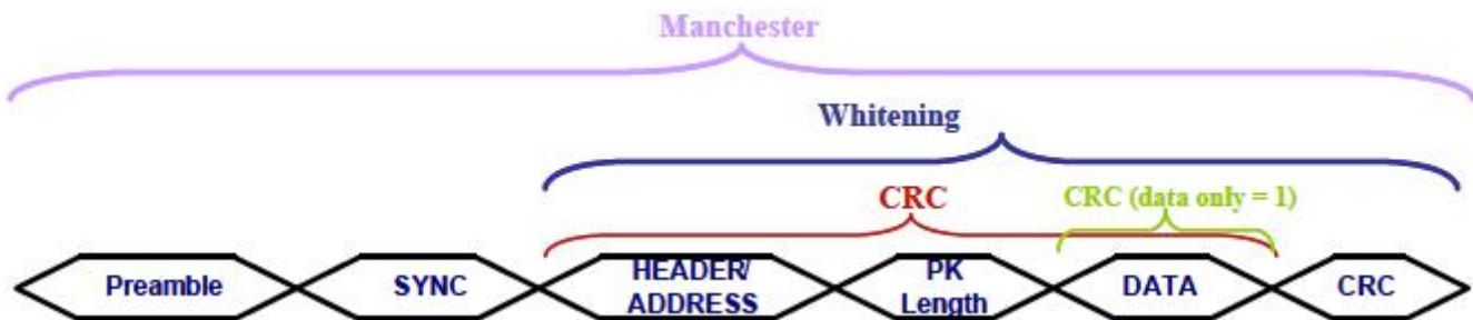
Figure 16. Operation of Data Whitening, Manchester Encoding, and CRC
