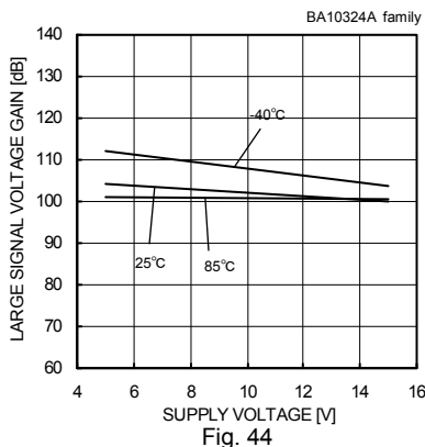
Large Signal Voltage Gain - Supply Voltage (RL=2[kΩ])
