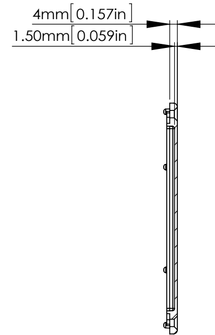
SECTION B-B
